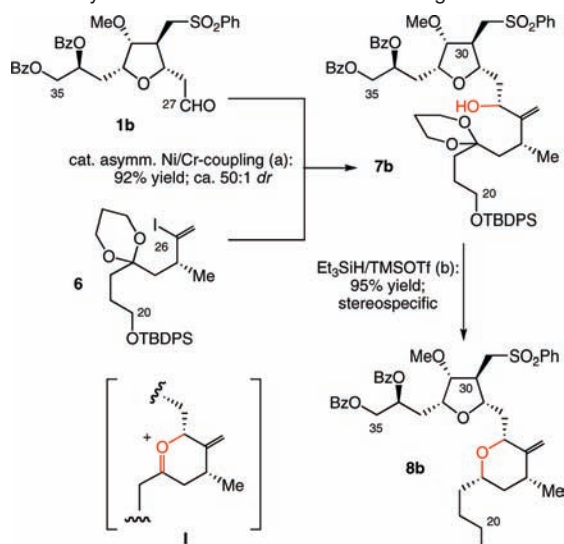
Scheme 3. Synthesis of E7389 C20–C35 Building Block 8b a
