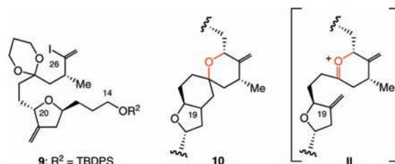
Scheme 4. Attempted Synthesis of E7389 C20–C35 Building Block 3b via the Oxonium Route
