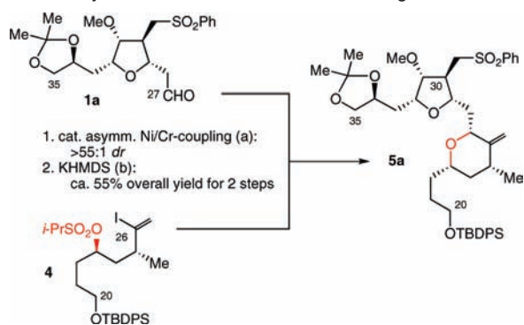
Scheme 2. Synthesis of E7389 C20–C35 Building Block 5a a
